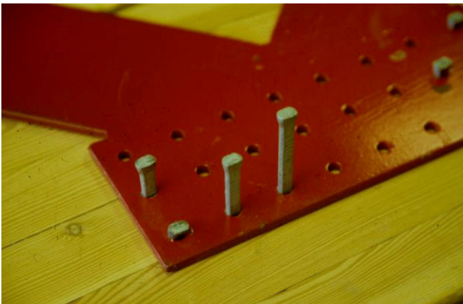
Figure 1. Detail of rivet connection showing perforated plate on 25 mm grid and shape of rivet at various stages of installation.
