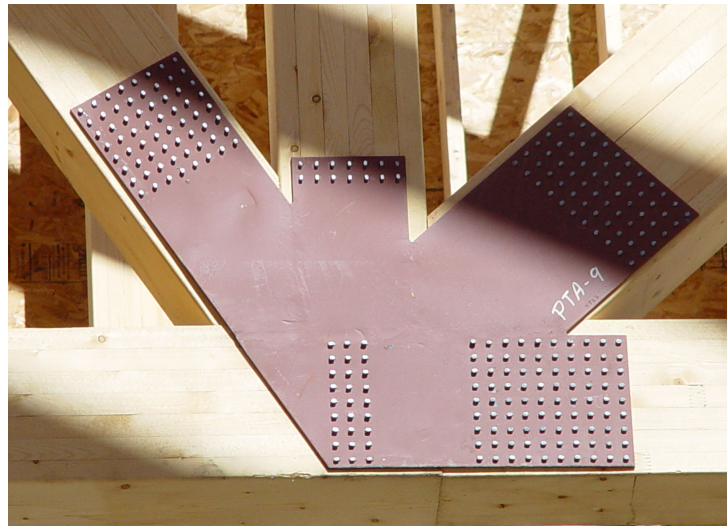
Figure 2. Rivet connection of a glulam truss (plate on other side as well). Note the alignment of the rivets with the grain direction.
